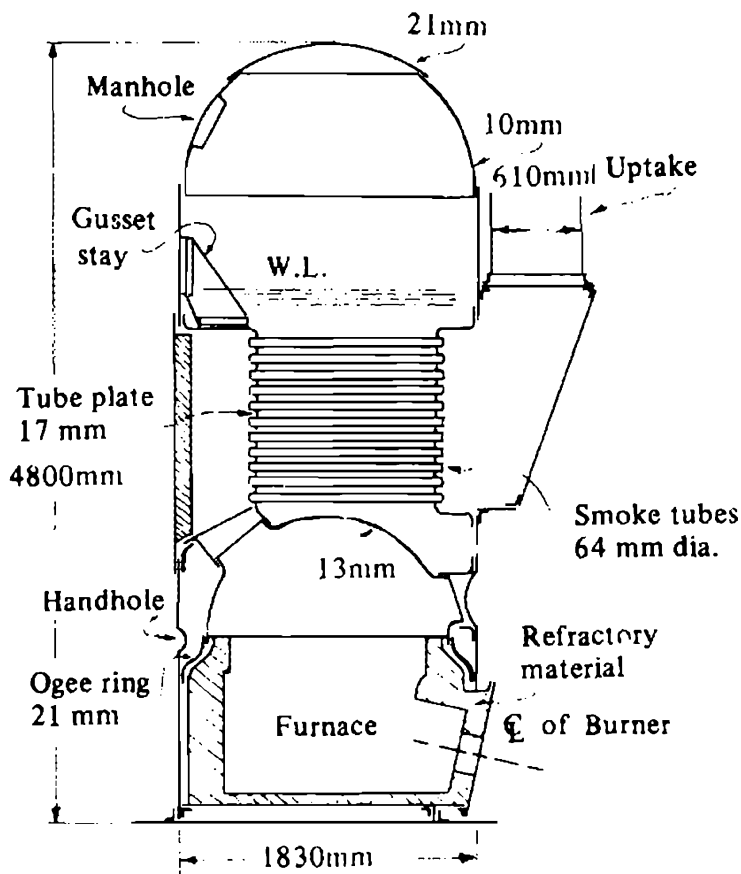
Fig. 17 Cochran smoke tube boiler
