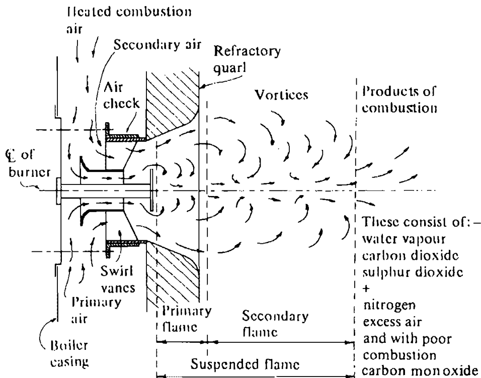
Fig. 70 Combustion in a boiler furnace
