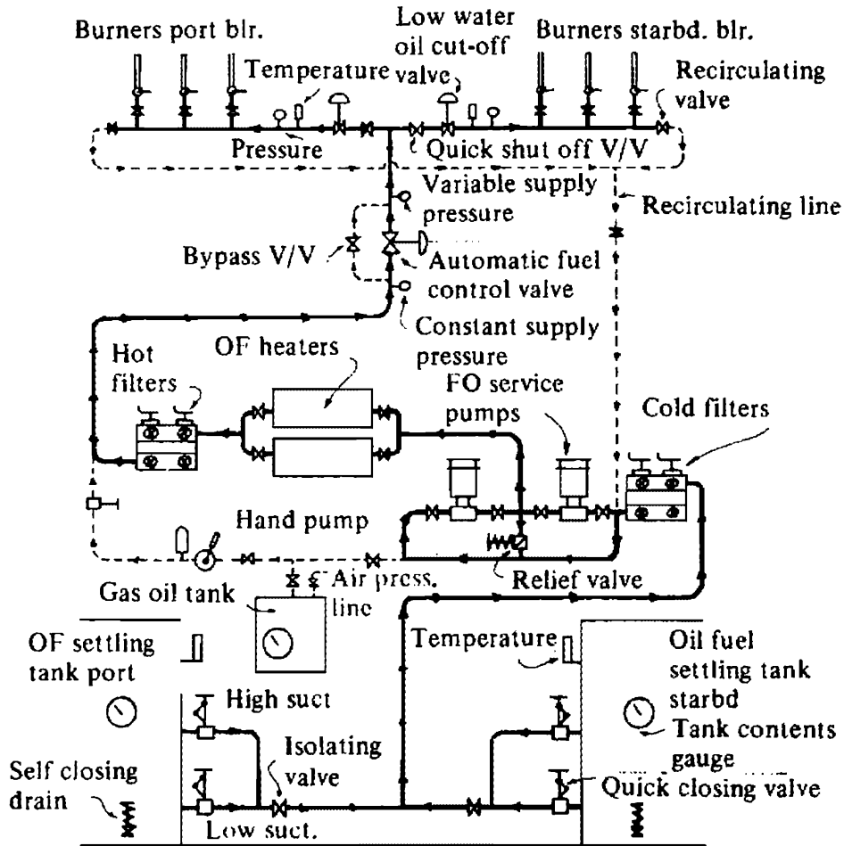
Fig. 77 Fuel oil system
