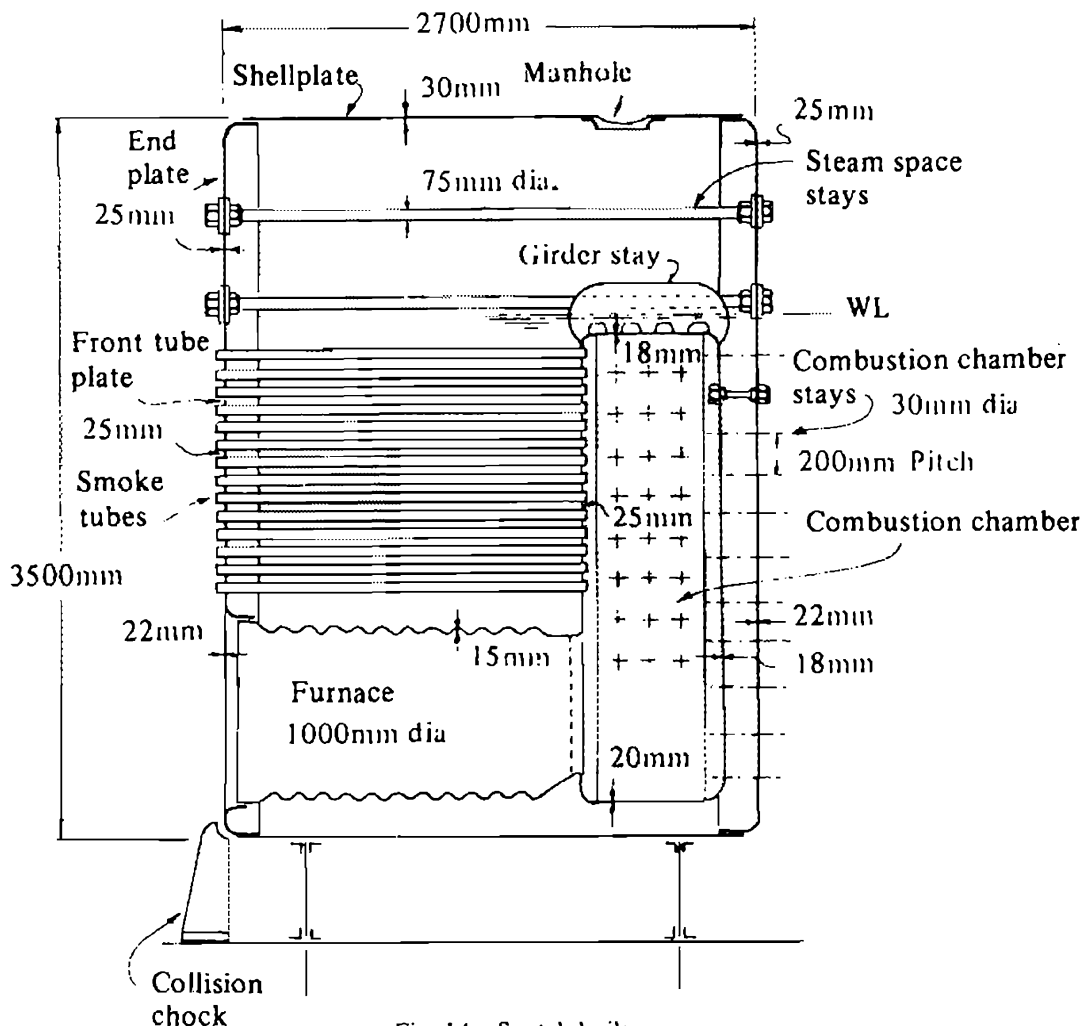
Fig. 14 Scotch boiler
