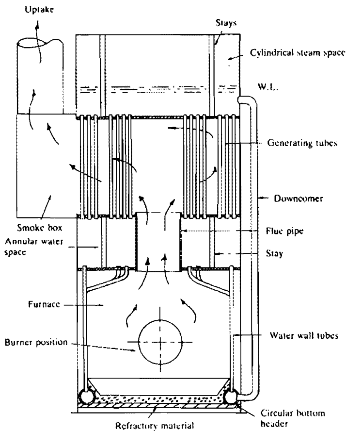
Fig. 21 Aalborg vertical water tube boiler
