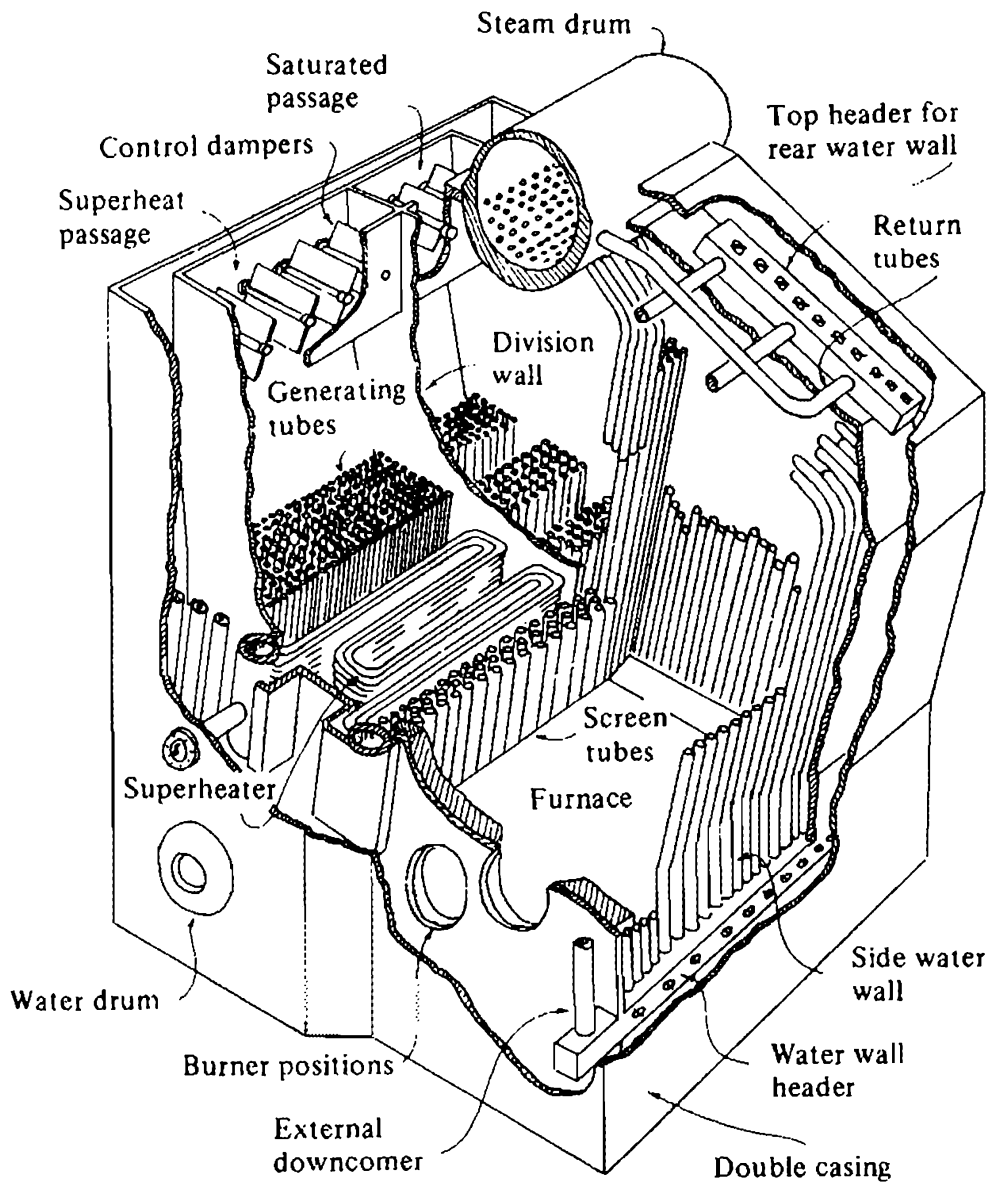
Fig. 33 Babcock and Wilcox selectable superheat boiler
