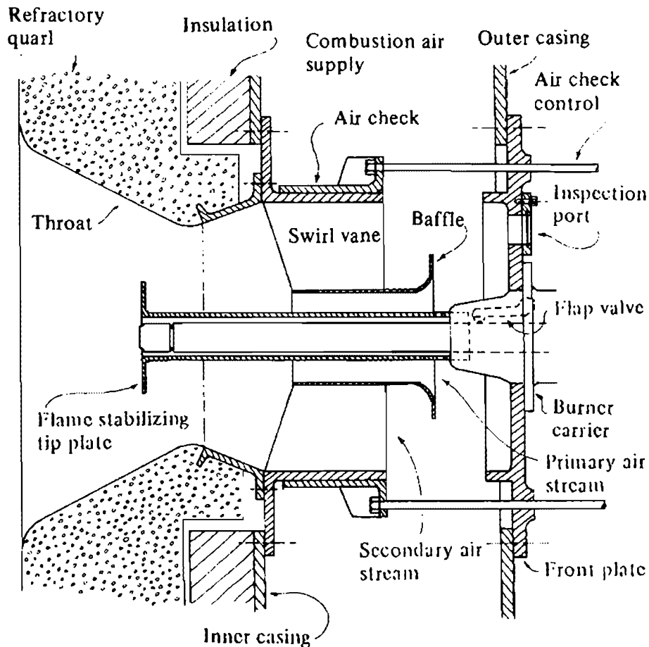
Fig. 76 Air register
