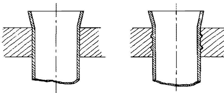
Grooved seat
