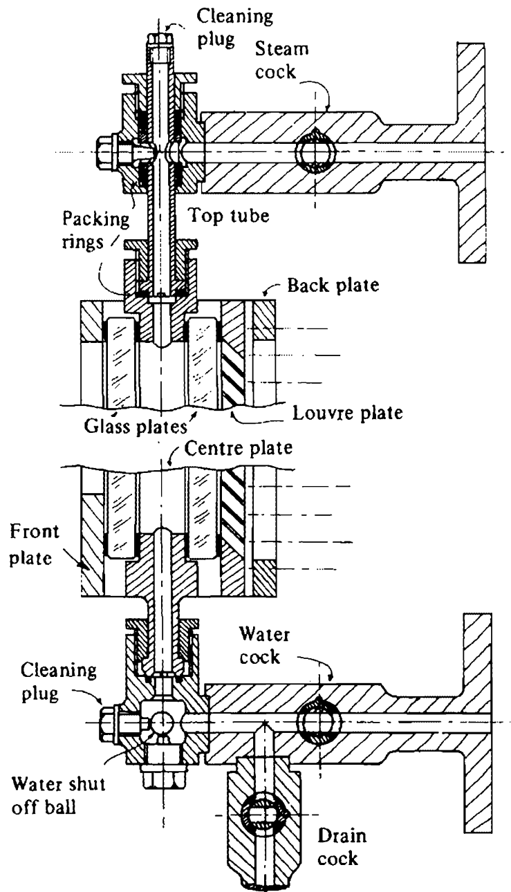
Fig. 58 Double plate type water level gauge
