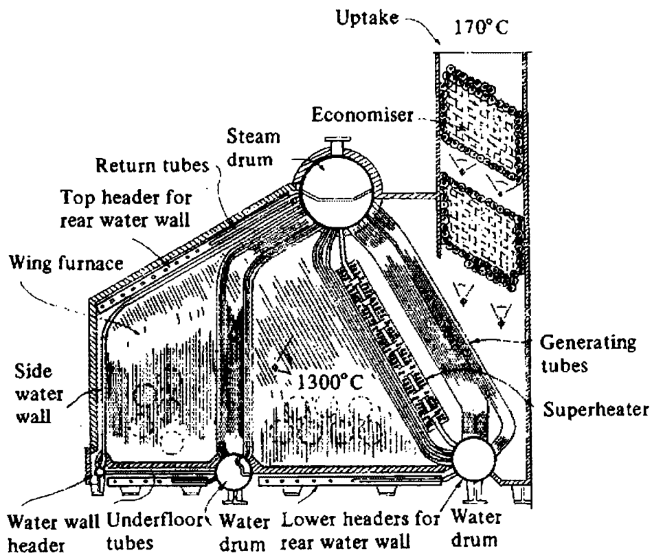
Fig. 32 Foster Wheeler controlled superheat boiler
