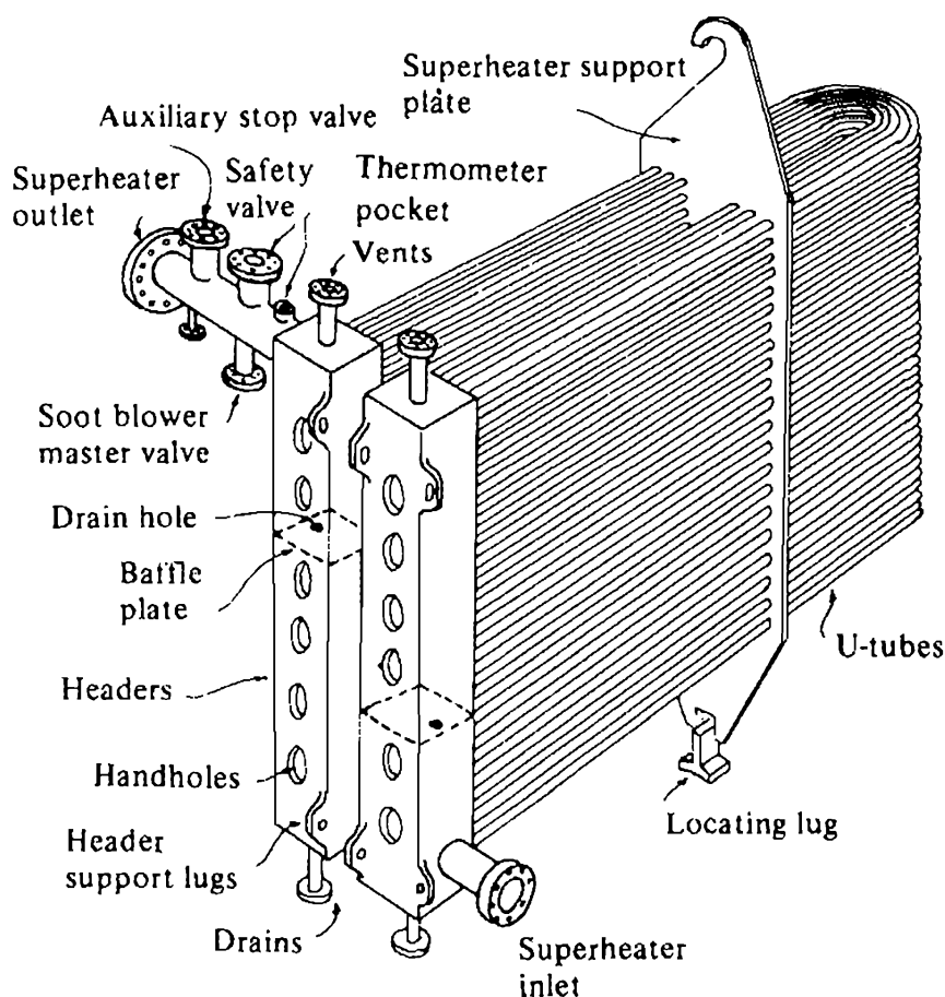
Fig. 44 Superheater in a D-type boiler
