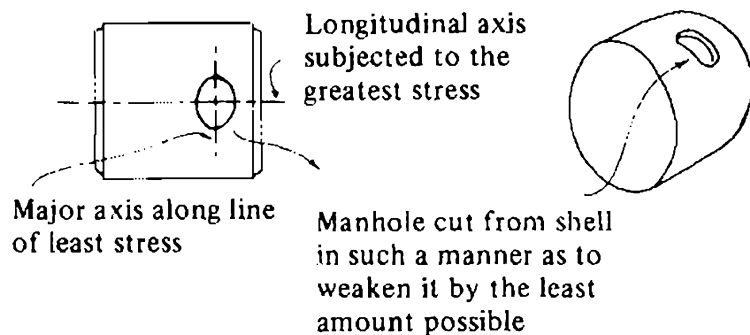
Fig. 6 Arrangement of manhole in a Scotch boiler shell
