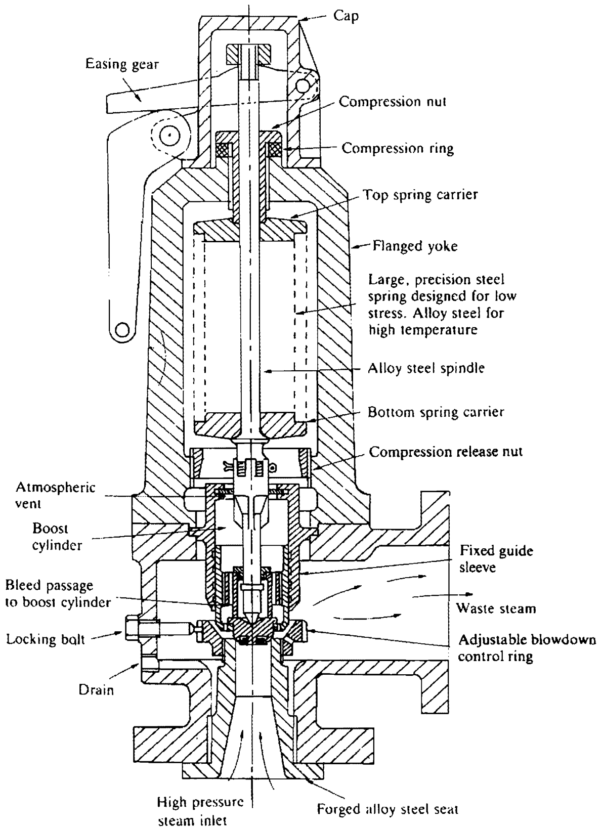
Fig. 69 Consolidated type safety valve
