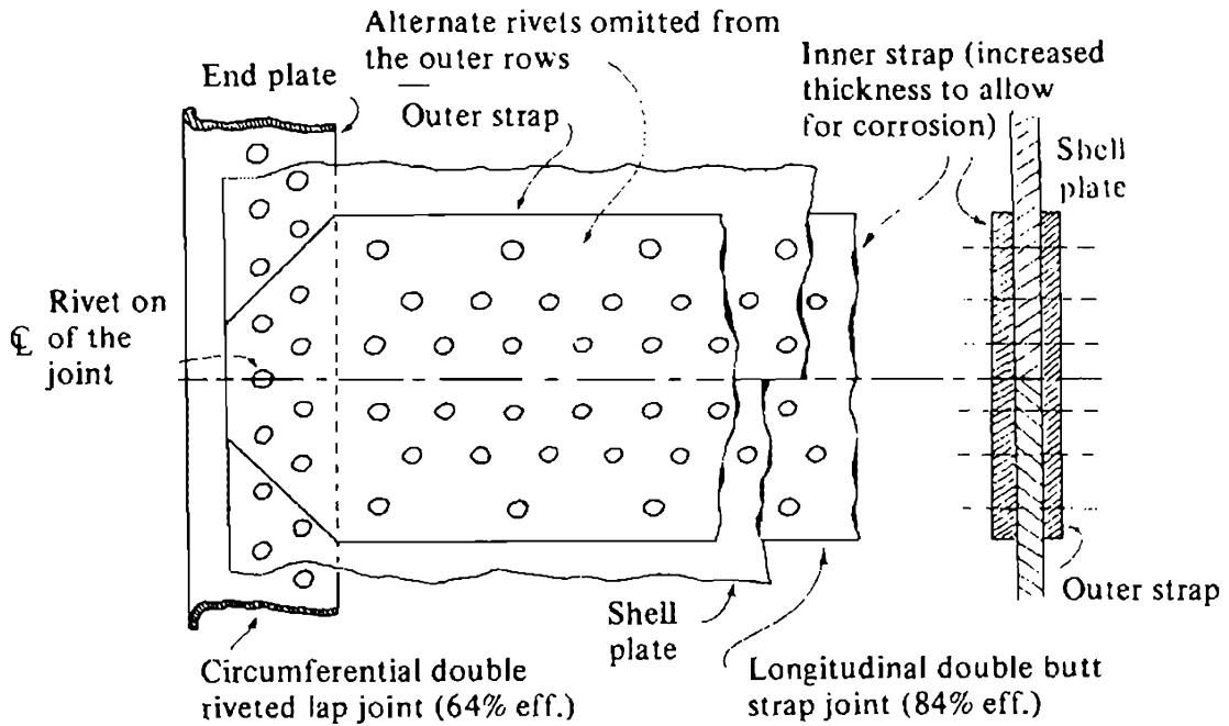
Fig. 4 Detail of riveted longitudinal joint
