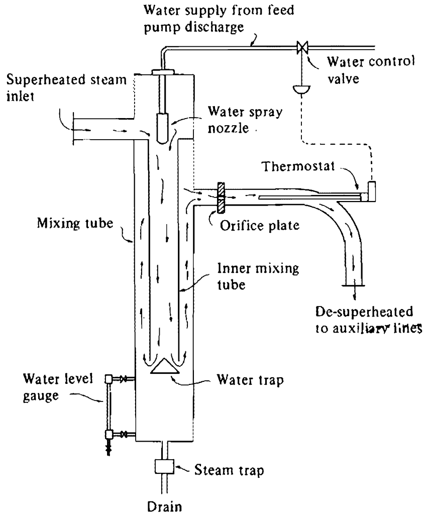
Fig. 51 Spray type de-superheater
