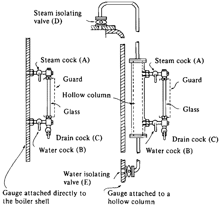
Fig. 56 Alternative arrangements of water level gauges
