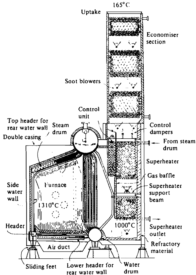
Fig. 35 Foster Wheeler ESD.11 boiler
