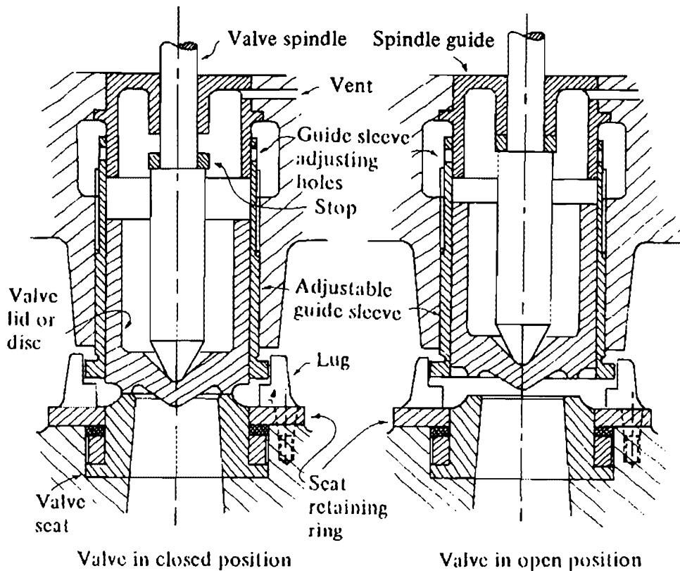
Fig. 68 Detail of full lift safety valve
