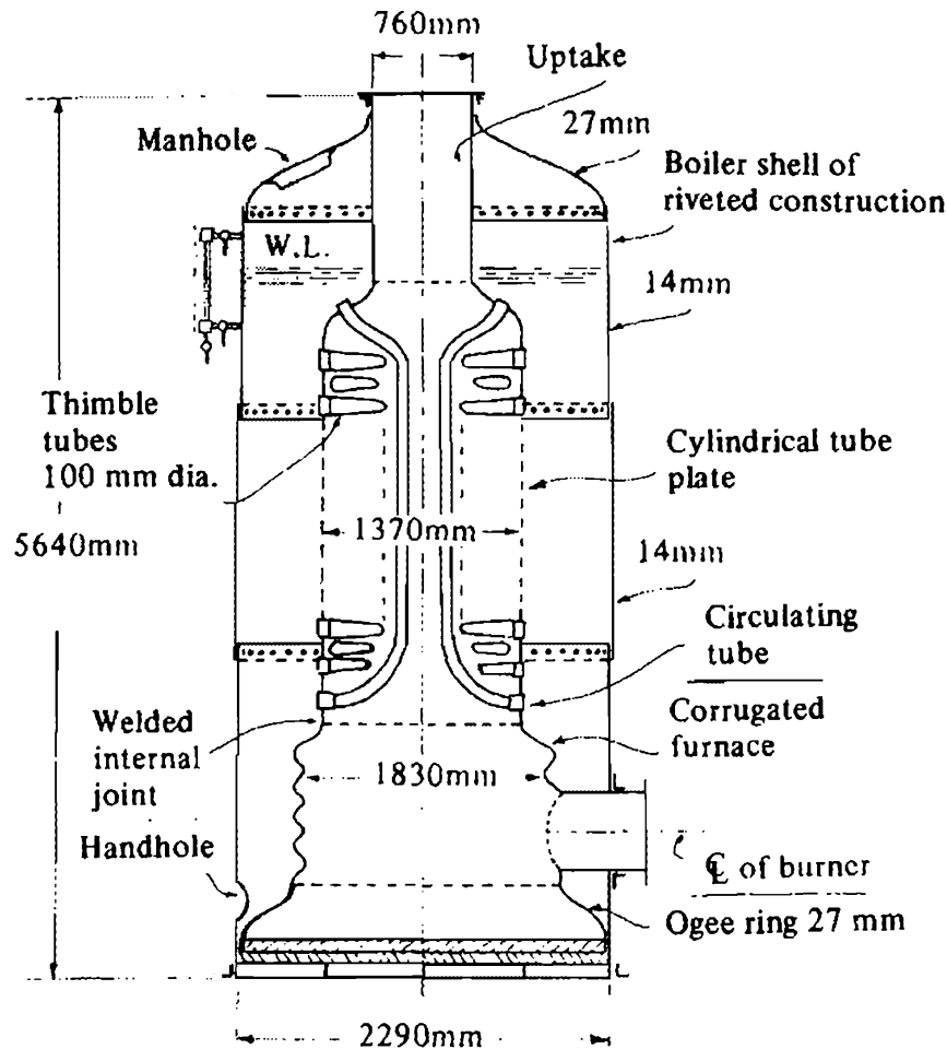
Fig. 19 Clarkson thimble tube boiler
