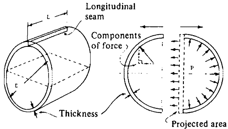
Fig. 1 Stress in the longitudinal seam
