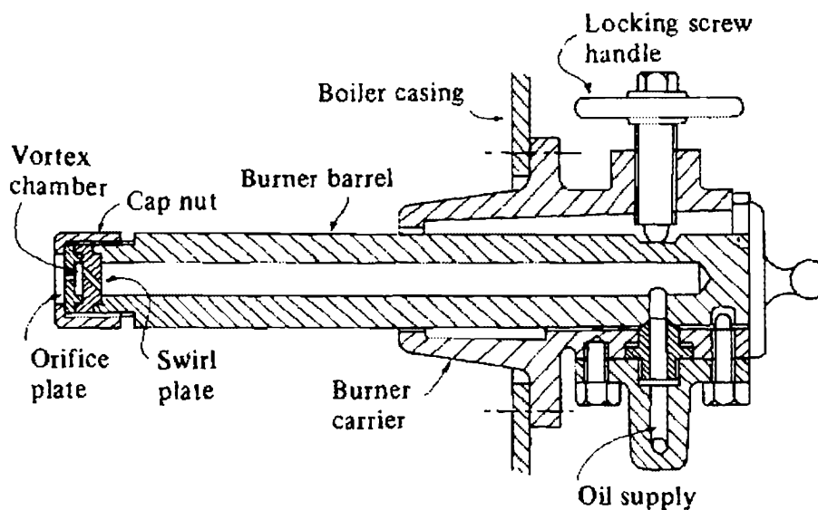
Fig. 71 Pressure jet type fuel oil burner
