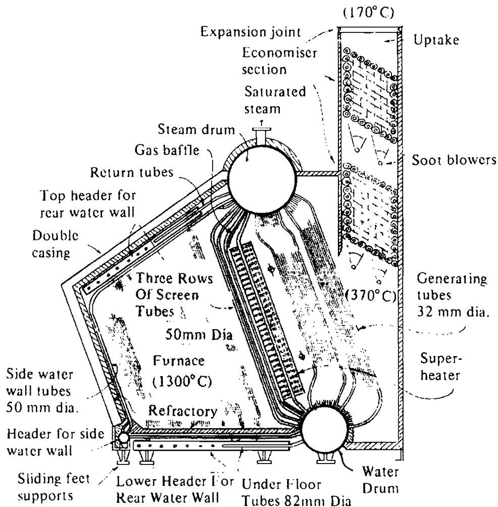
Fig. 31 Foster Wheeler D-type boiler
