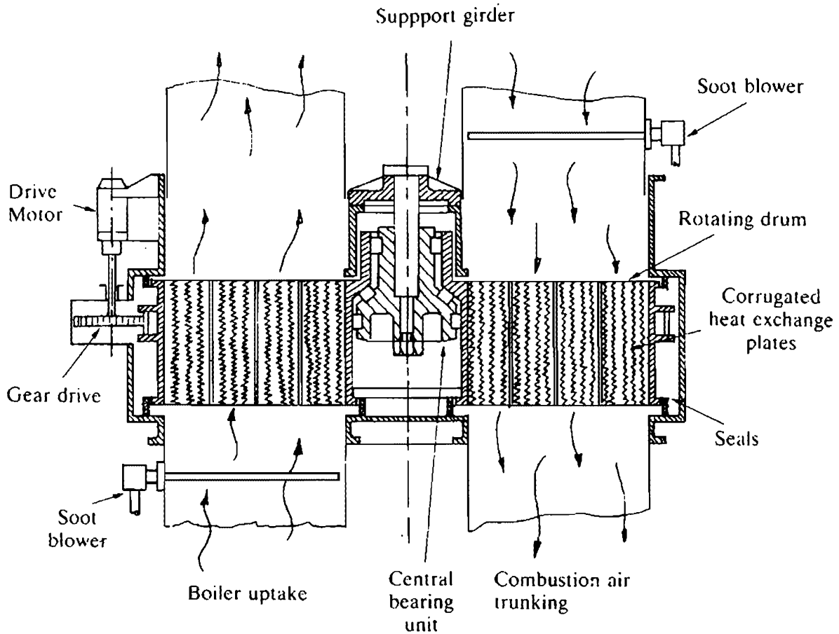
Fig. 54 Rotary type air heater
