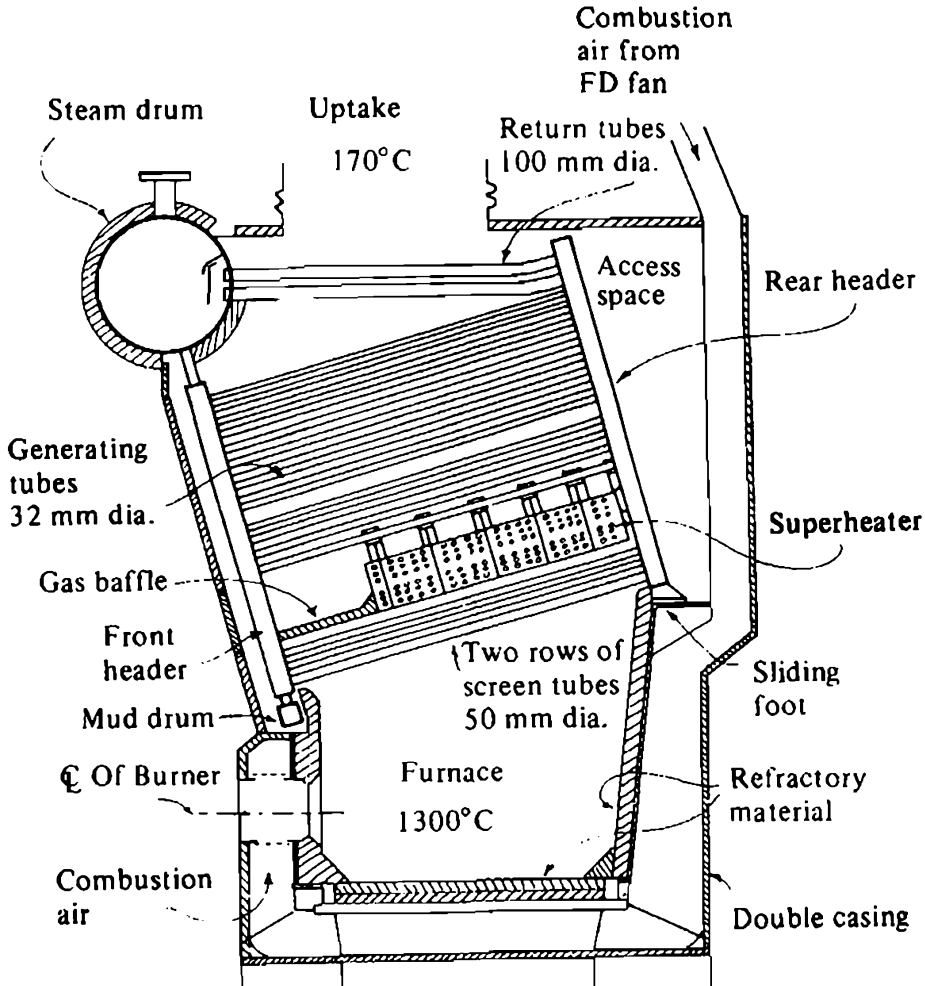
Fig. 30 Babcock and Wilcox header boiler
