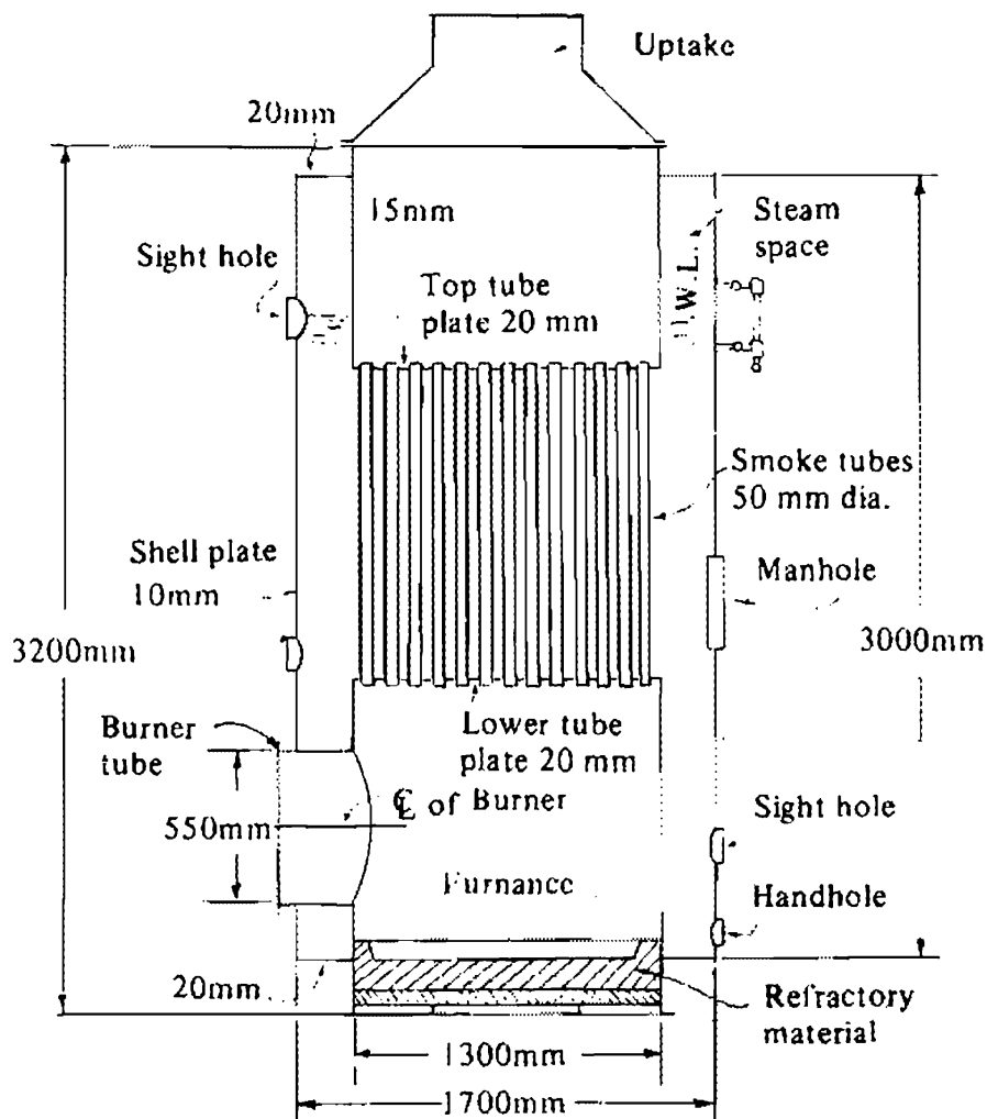
Fig. 20 Spanner vertical smoke tube boiler
