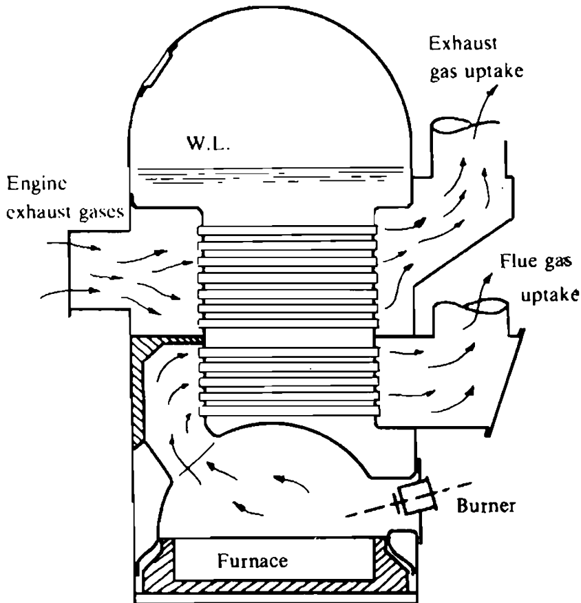
Fig. 26 Composite boiler
