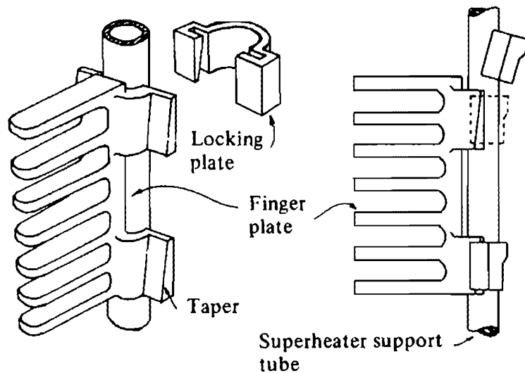
Fig.47 Finger plate type tube supports
