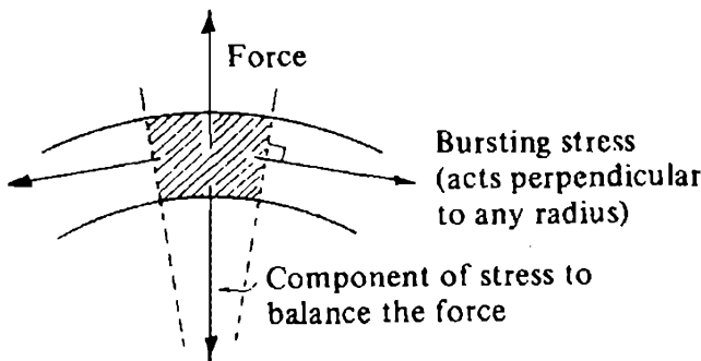
Fig. 9 Stress in a curved plate
