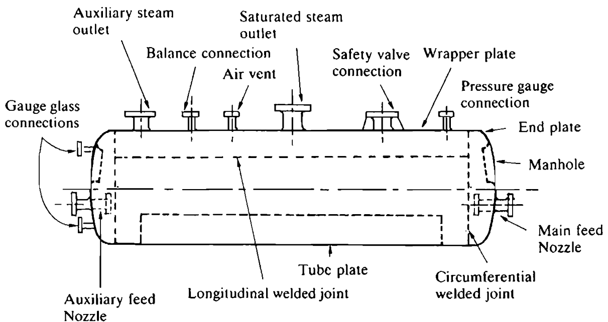
Fig 29. Steam drum for a water tube boiler
