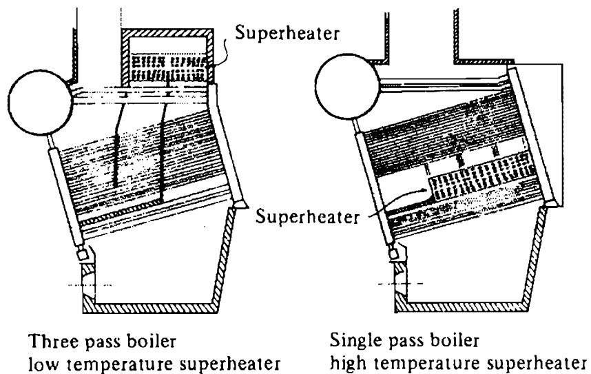
Fig. 43 Alternative superheater positions in header boilers
