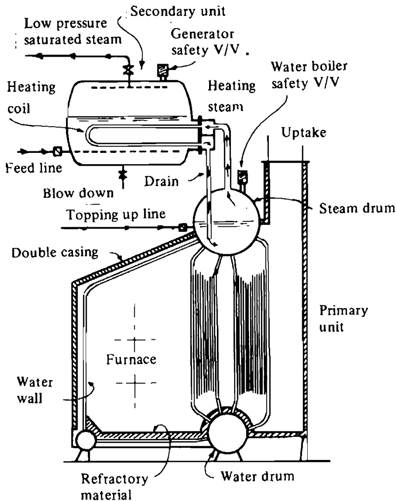
Fig. 25 Dual pressure boiler
