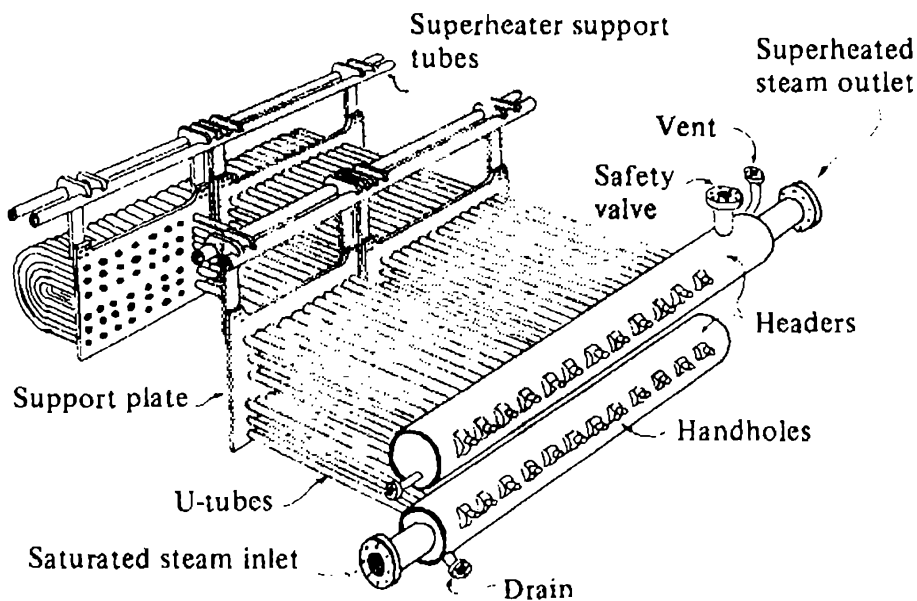
Fig. 42 Superheater in a header boiler
