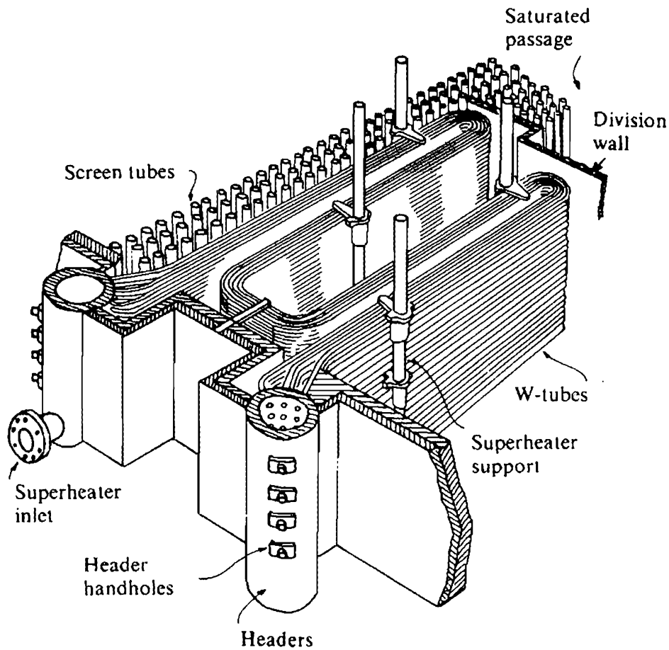
Fig. 46 Superheater in a selectable superheat boiler
