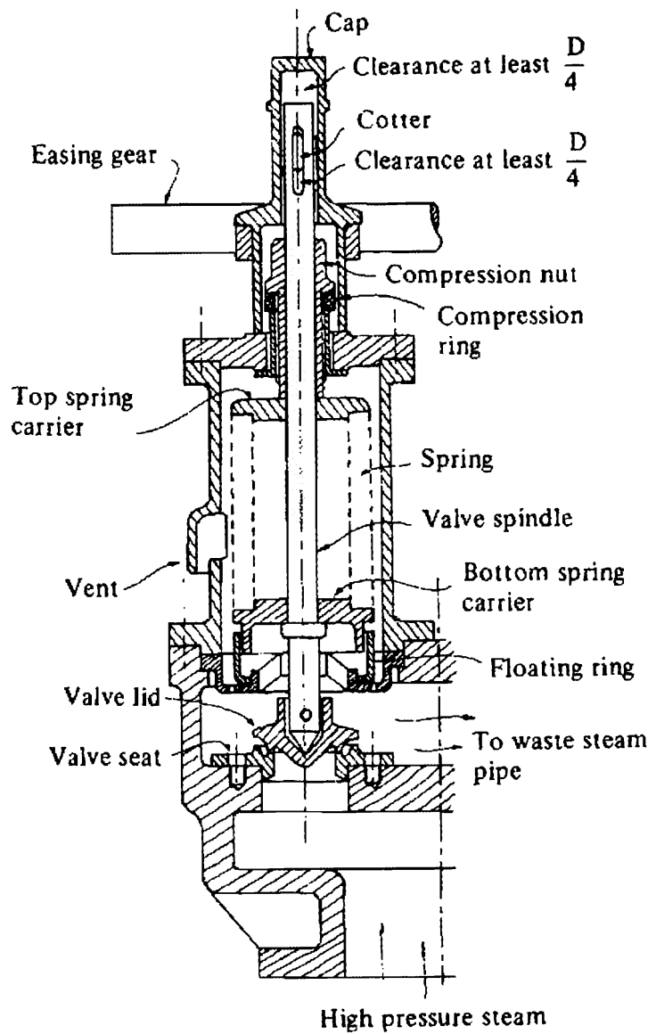
Fig. 64 Improved high lift safety valve
