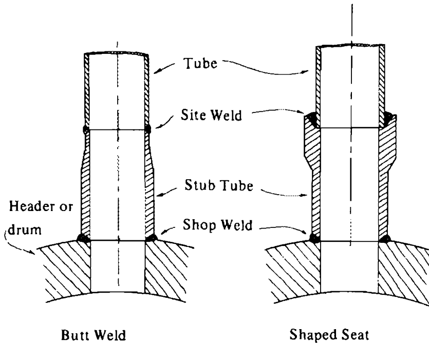
Fig. 39 Welded tube attachment
