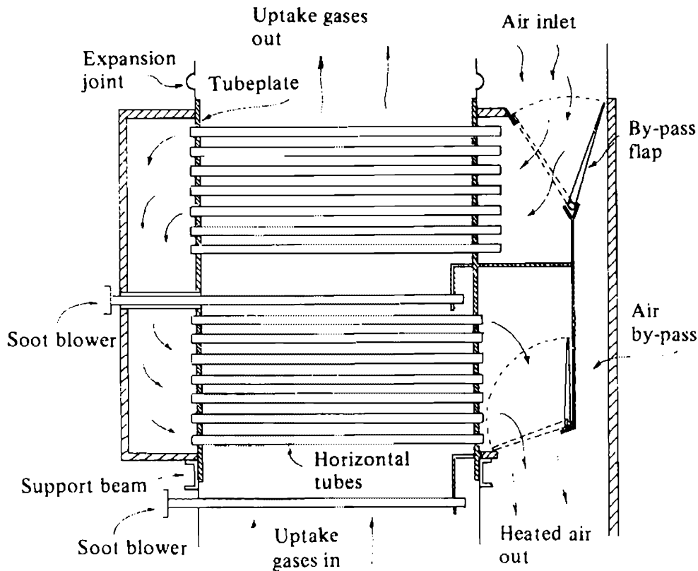
Fig. 53 Tubular type air heater
