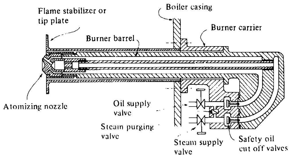
Fig. 74 Steam blast jet type fuel oil burner
