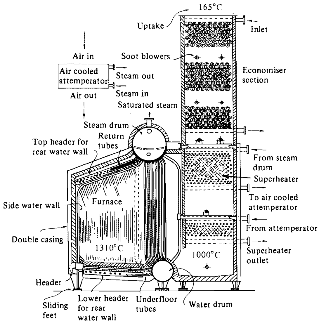
Fig. 34 Foster Wheeler ESD.1 boiler
