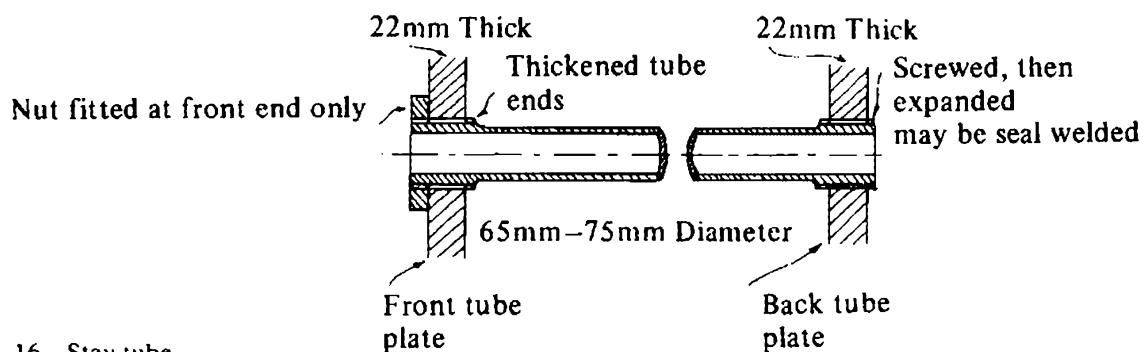
Fig. 16 Stay tube
