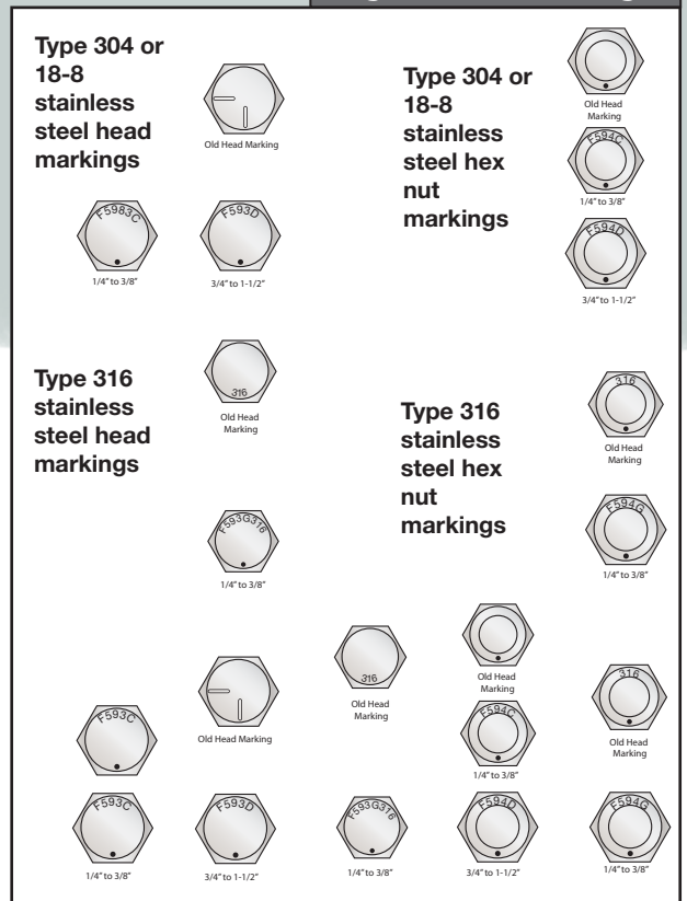
Figure 1 - Head Markings
