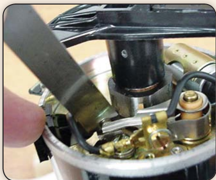
Setting point gap with a feeler gauge.
