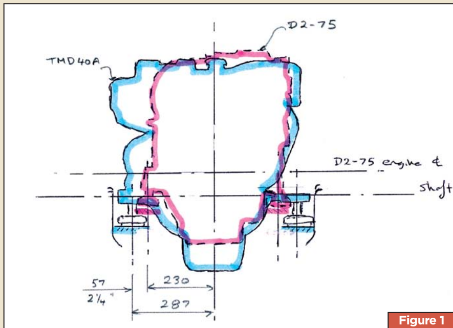
Outline sketches of new (pink line) and old (blue line) engines.
