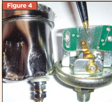
Figure 4 Cut open sensor showing wiper and broken resistance wire.
