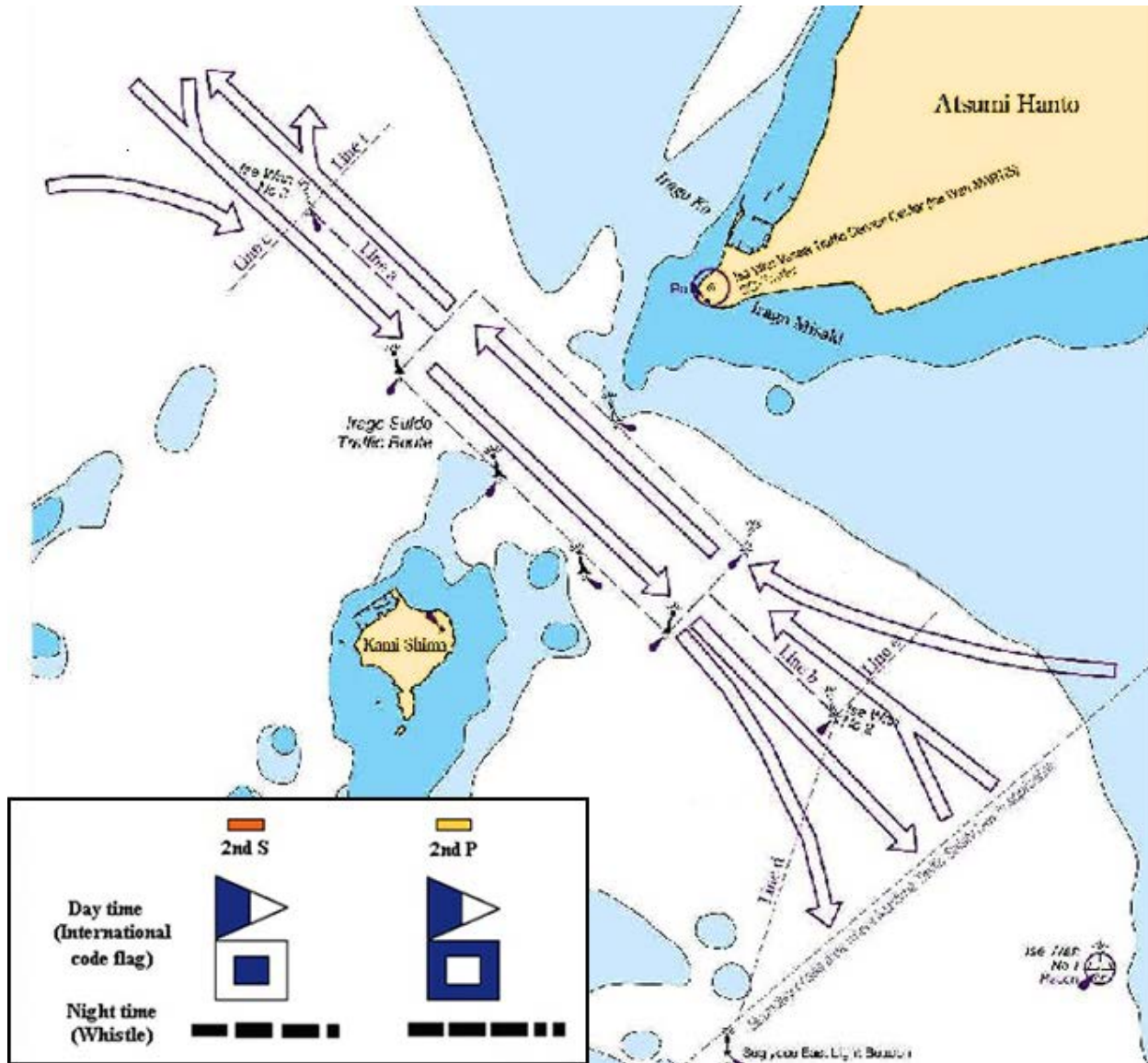
Irago Suido—Traffic Lanes and Signals
